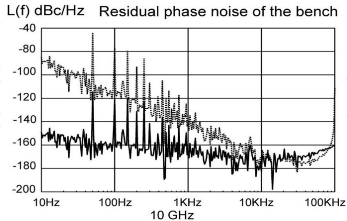
Figure 5. Phase noise floor (dBc/Hz) of the bench measured at 10 GHz with Anritsu synthesizer (500 averages) versus Fourier Frequency between 10 Hz and 100 kHz.
