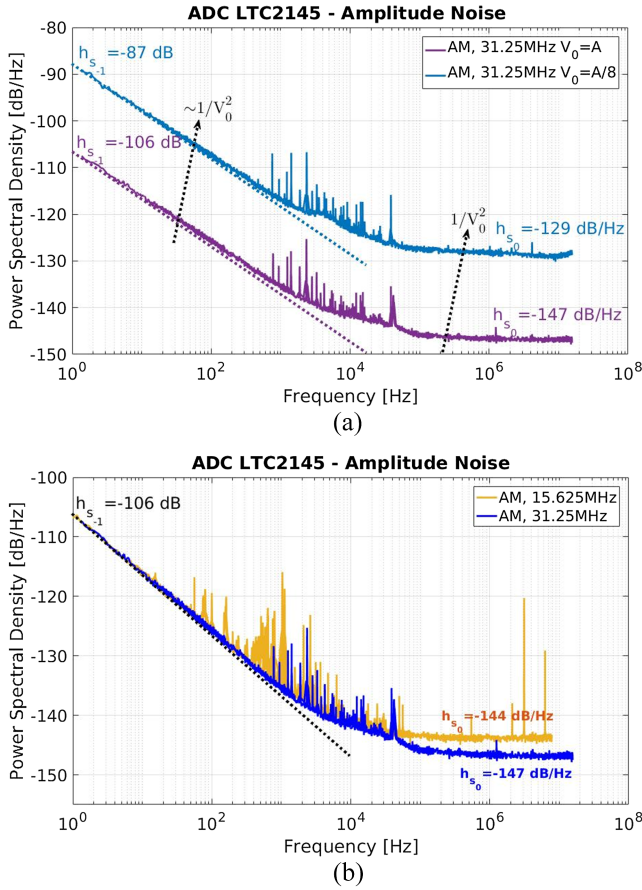
FIG. 12. (a) ADC Amplitude noise dependency with respect to input amplitude. (b) AM noise dependency with respect to input frequency. In agreement with the ADC noise model, the ADC amplitude noise is dependent on the input amplitude and independent of the input frequency. The noise is dominated by the fluctuations generated by the additive noise of the input stage, which causes similar effects on the ADC phase and amplitude noise.
