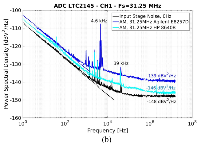
FIG. 10. (a) AM in common mode. ADC AM noise comparison using two signal generators. The amplitude noise generated by the ADC was estimated at the maximum amplitude points of the sine-wave input signal where the effects of this noise are higher. (b) AM in single channel - Channel 1.
