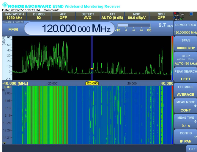
Fig. 13 Wide bandwidth waterfall (courtesy: R & S)
