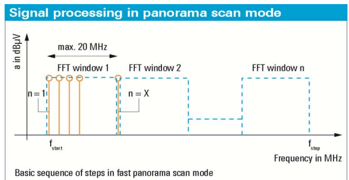
Fig. 5 Signal Processing in Panorama scan mode
