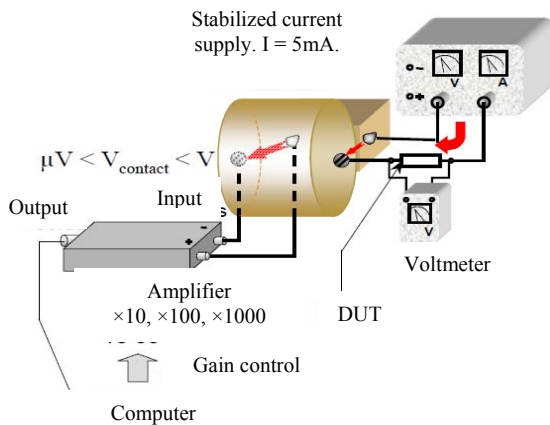
Fig. 3. Principle of 4-wire electrical contact resistance measurement [2]
