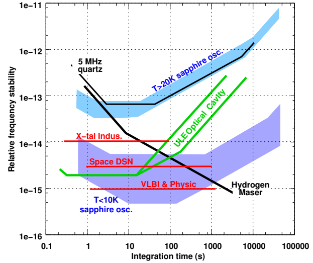
Figure 1. Relative frequency stability of some clocks and oscillators.
