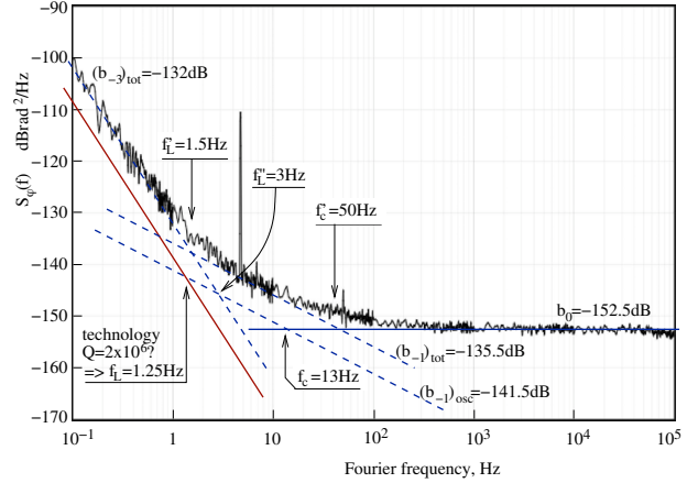
Fig. 5. Phase noise of the CMAC Pharo 5 MHz quartz OCXO. Courtesy of CMAC. Interpretation and mistakes are of the authors.
