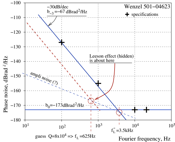
Fig. 6. Phase noise of the Wenzel 501-04623 100 MHz quartz OCXO [37].
