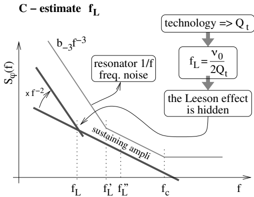
Fig. 4. Interpretation of the phase noise in quartz oscillators.
