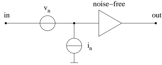
Figure 10: Rothe-Dahlke model of the noisy amplifier.
